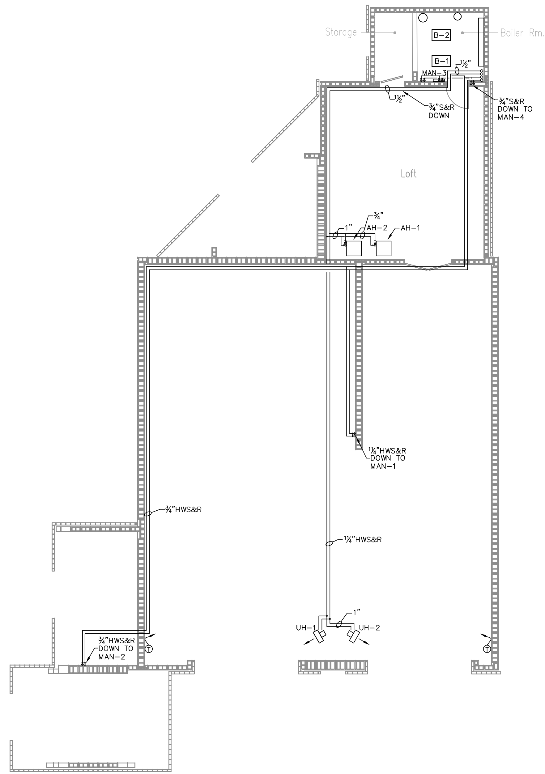
LOFT FLOOR PLAN SCALE: 1/8" = 1'-0"
