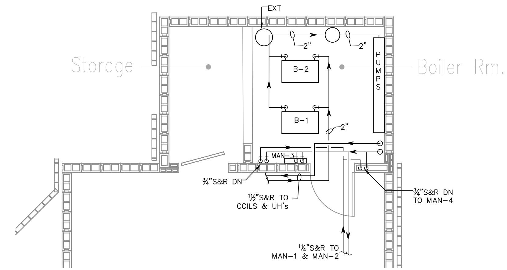
BOILER ROOM PART PLAN SCALE: 1/4" = 1'-0"
